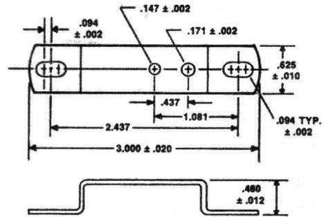
2014-0020 Mounting Kit For Stud Mount Relays
