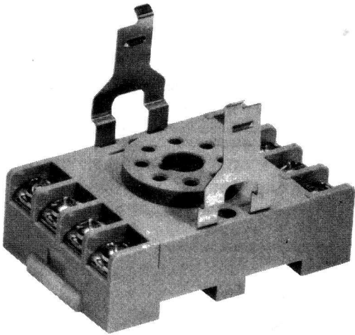
60SFA201 Clips ONLY Shown Assembled in Socket 2 Required Per Socket
